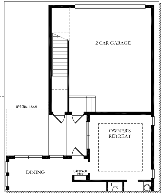
FIRST FLOOR WITH OPTIONAL RETREAT ABOVE
