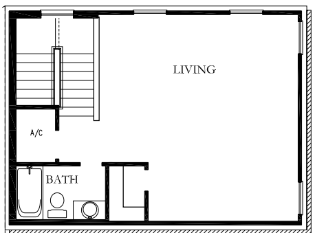
OPTIONAL RETREAT AT GARAGE WITH BATH
