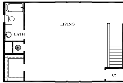
3 CAR DETACHED GARAGE W/OPT. RETREAT W/BATH
