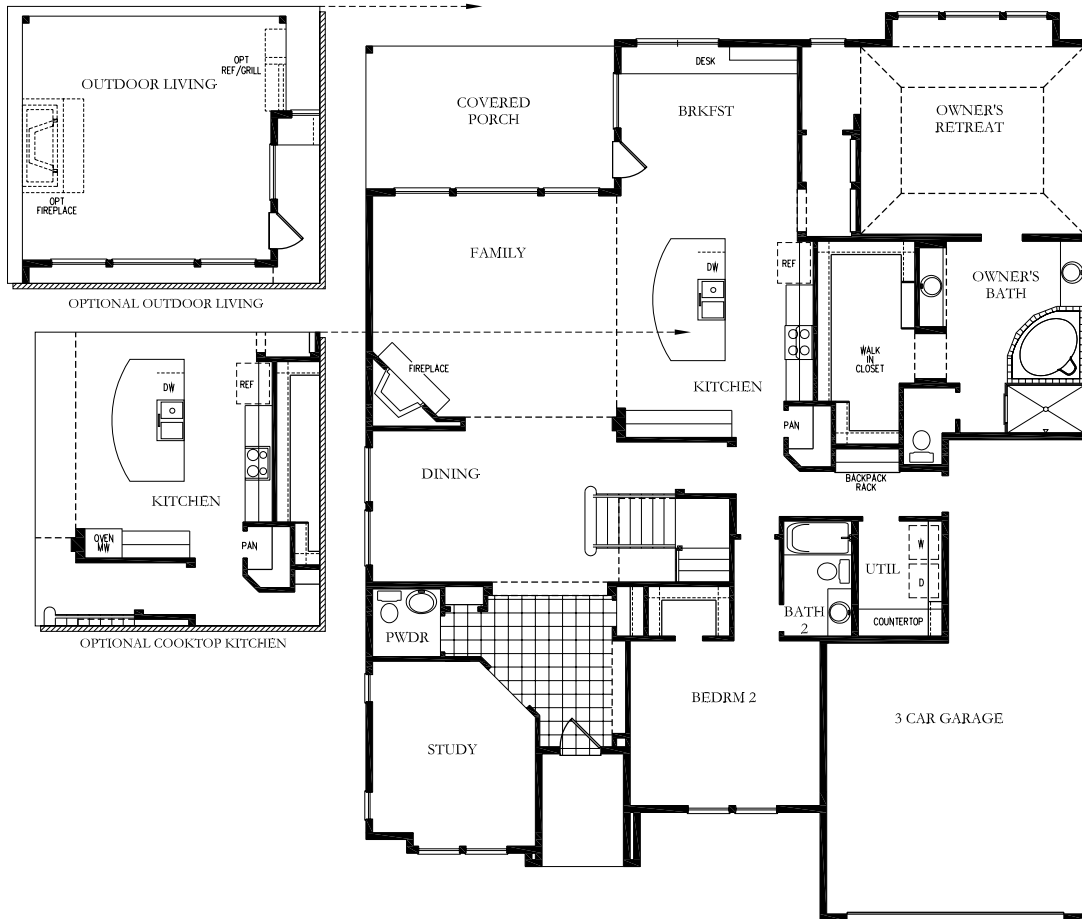
FIRST FLOOR
