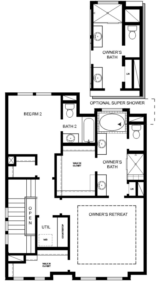
THIRD FLOOR
