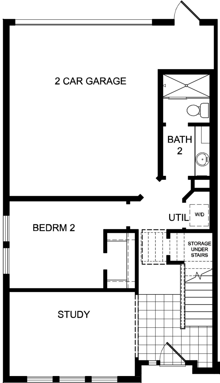
FIRST FLOOR
