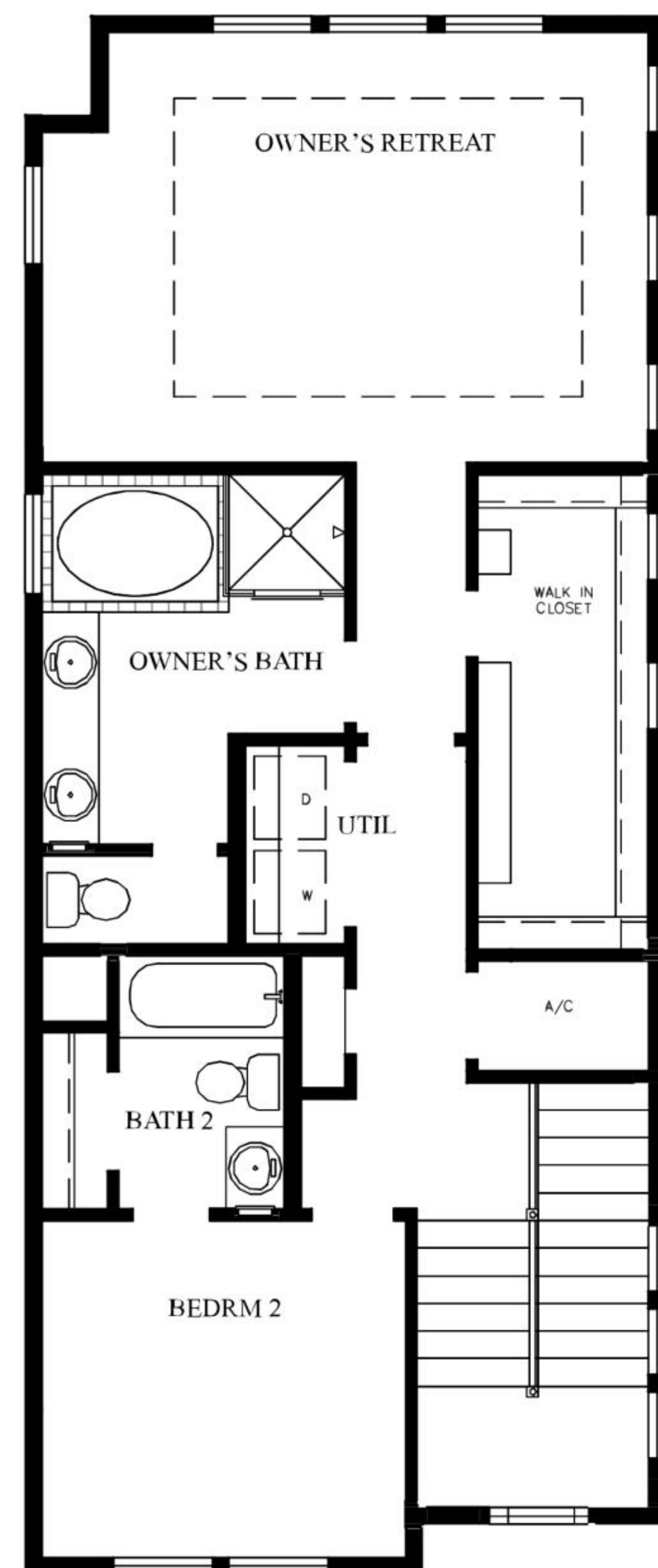
SECOND FLOOR
