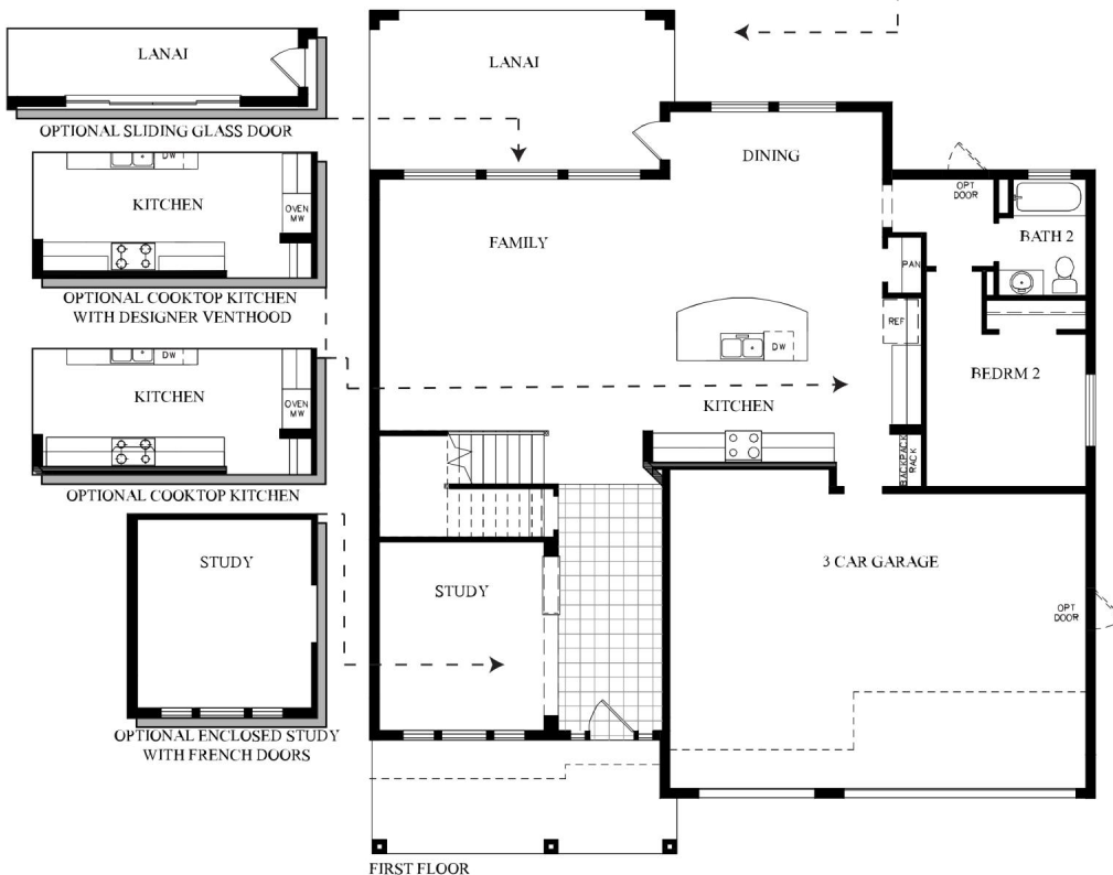
FIRST FLOOR
