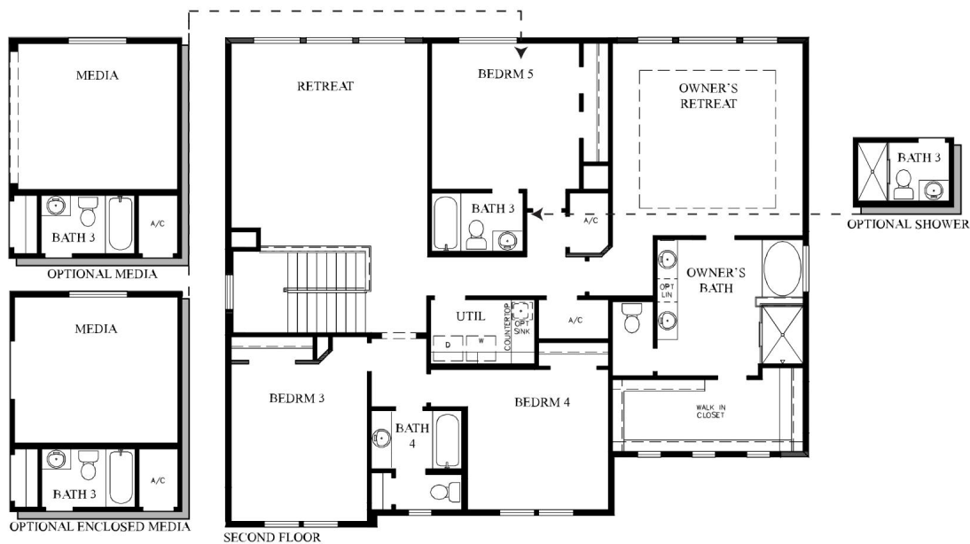
SECOND FLOOR
