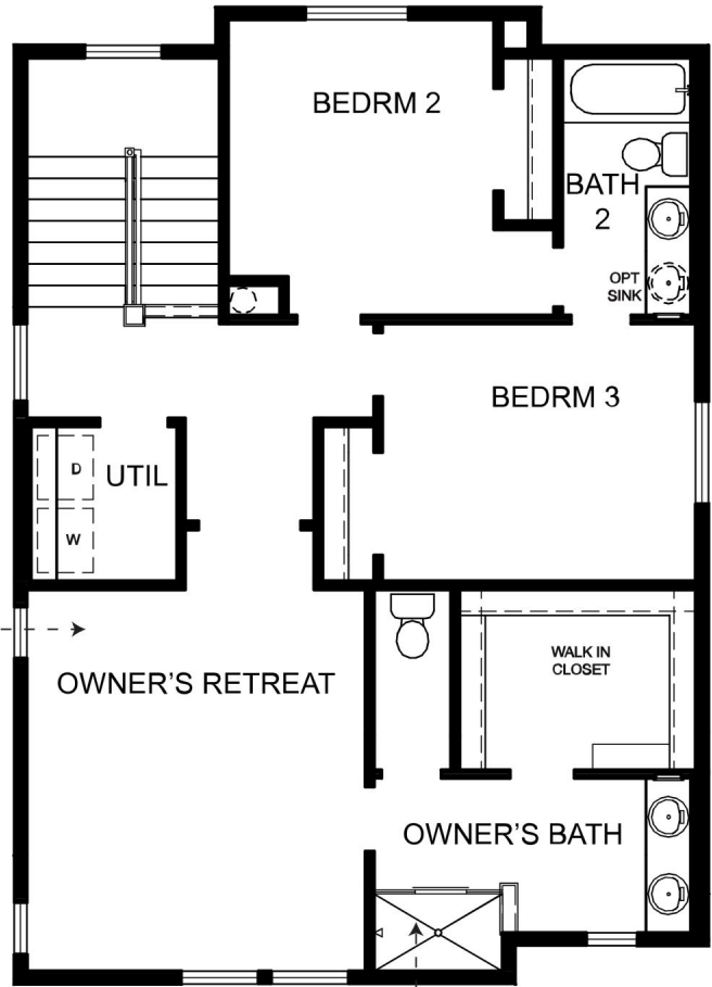
SECOND FLOOR
