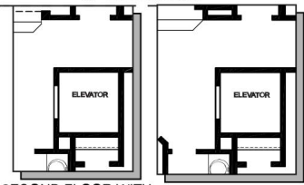
SECOND FLOOR WITH OPTIONAL ELEVATOR SECOND FLOOR WITH OPTIONAL ELEVATOR WITH OPTIONAL MEDIA
