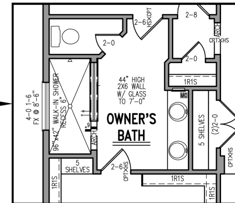
EXAMPLE SUPER SHOWER LAYOUT
