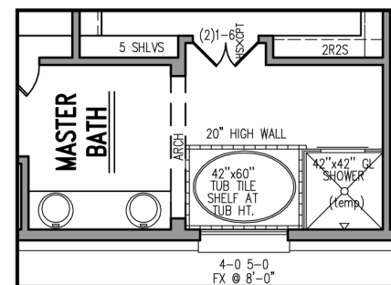
EXAMPLE TUB/SHOWER LAYOUT
