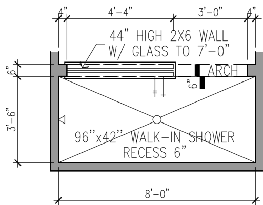
TYPICAL SUPER SHOWER
