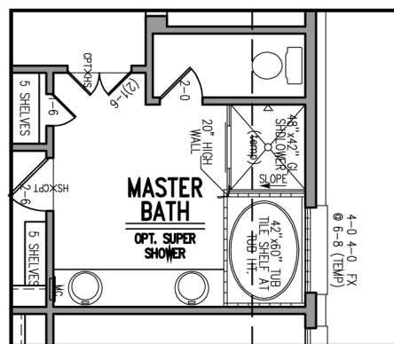
EXAMPLE TUB/SHOWER LAYOUT
