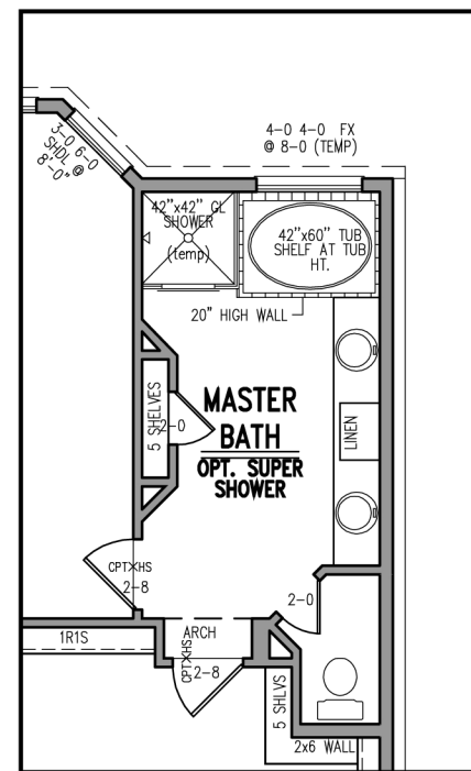
EXAMPLE TUB/SHOWER LAYOUT
