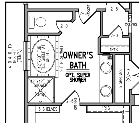
EXAMPLE TUB/SHOWER LAYOUT
