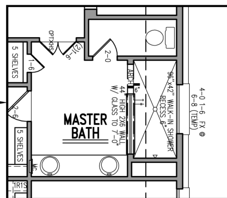
EXAMPLE SUPER SHOWER LAYOUT
