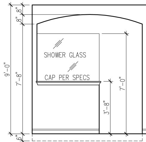
TYPICAL ARCH SUPER SHOWER
