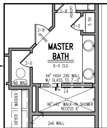
EXAMPLE SUPER SHOWER LAYOUT
