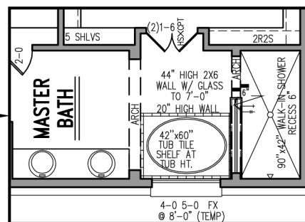
EXAMPLE SUPER SHOWER LAYOUT
