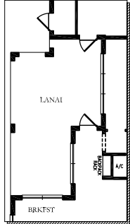
OPTIONAL EXTENDED LANAI WITH RETREAT ABOVE GARAGE
