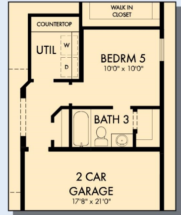
OPTIONAL BEDROOM 5 WITH BATH 3
