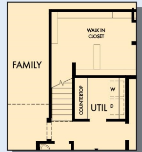
FIRST FLOOR WITH OPTIONAL SECOND FLOOR
