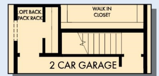
FIRST FLOOR WITH OPTIONAL SECOND FLOOR WALK UP ATTIC STORAGE
