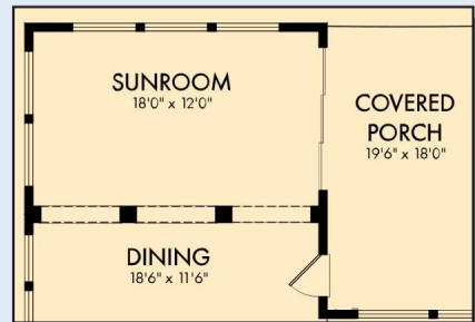
OPTIONAL SUNROOM WITH EXTENDED COVERED PORCH
