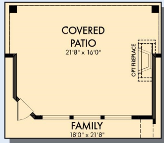
OPTIONAL EXTENDED COVERED PATIO
