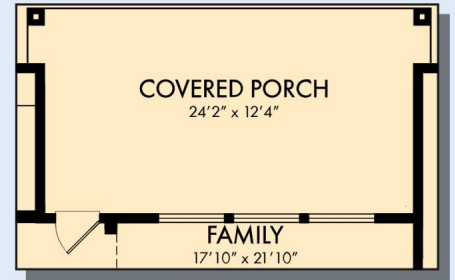
OPTIONAL EXTENDED COVERED PORCH AT FAMILY
