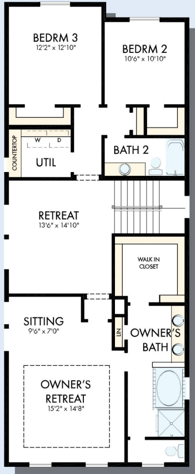
SECOND FLOOR
