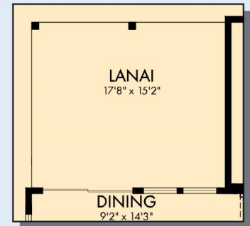
OPTIONAL EXTENDED LANAI WITH SLIDING GLASS DOOR AT DINING
