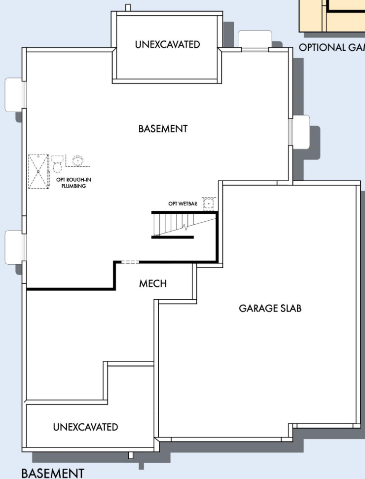
OPTIONAL DAYLIGHT AT BASEMENT
