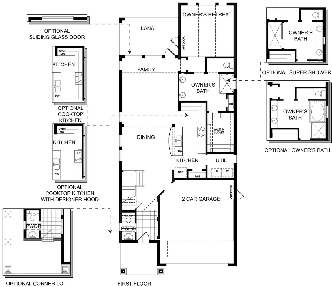
FIRST FLOOR
