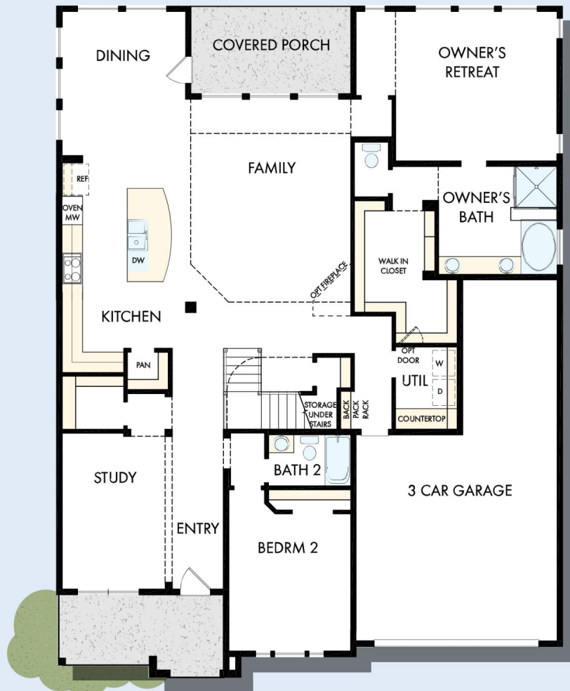
FIRST FLOOR
