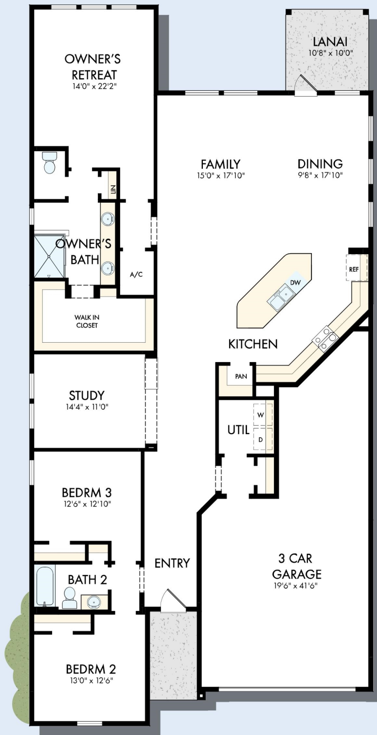
OPTIONAL SLIP IN TUB WITH SEPARATE SHOWER AT OWNER'S BATH
