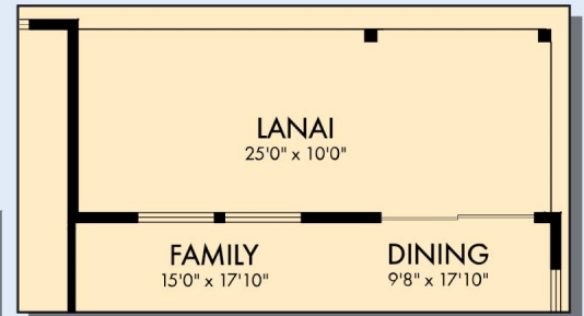
OPTIONAL EXTENDED LANAI WITH SLIDING GLASS DOOR AT FAMILY AND DINING
