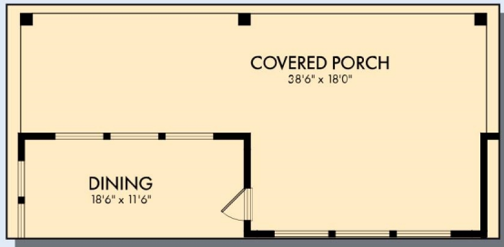
OPTIONAL EXTENDED COVERED PORCH
