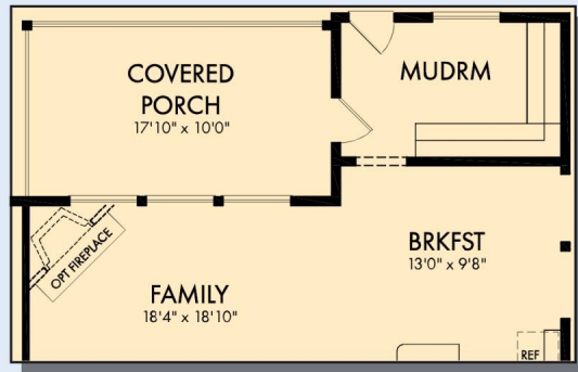
OPTIONAL MUDROOM AT COVERED PORCH
