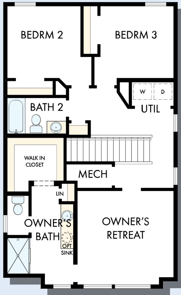
SECOND FLOOR
