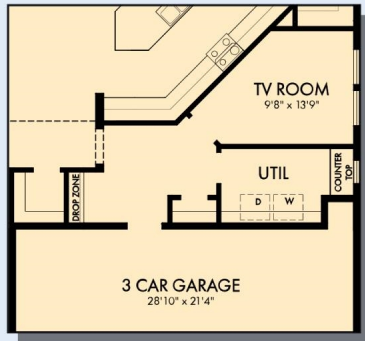
OPTIONAL TV ROOM AT GARAGE
