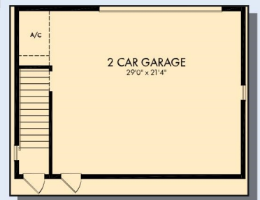
OPTIONAL DETACHED 2 CAR GARAGE WITH OPTIONAL RETREAT
