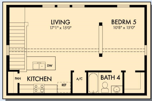
OPTIONAL SECOND FLOOR GARAGE RETREAT WITH BEDROOM 5 AND BATH 4 ABOVE 3 CAR GARAGE
