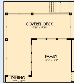
OPTIONAL EXTENDED COVERED DECK WITH DAYLIGHT/WALKOUT BASEMENT
