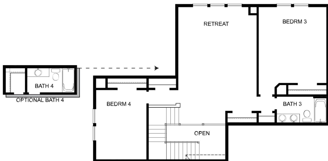
SECOND FLOOR
