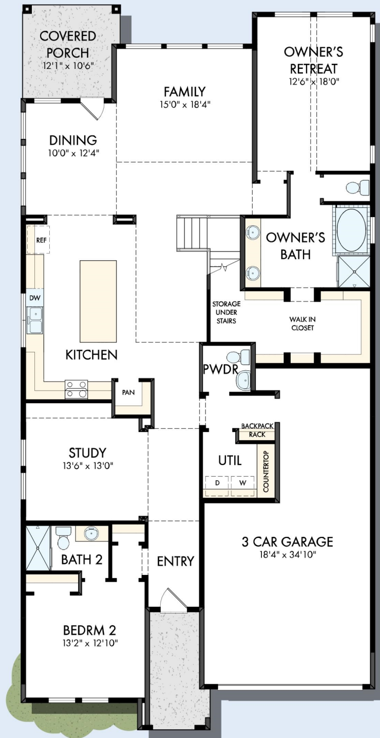
FIRST FLOOR
