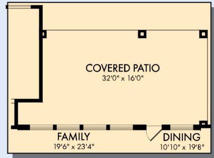
OPTIONAL EXTENDED COVERED PATIO AT FAMILY AND DINING
