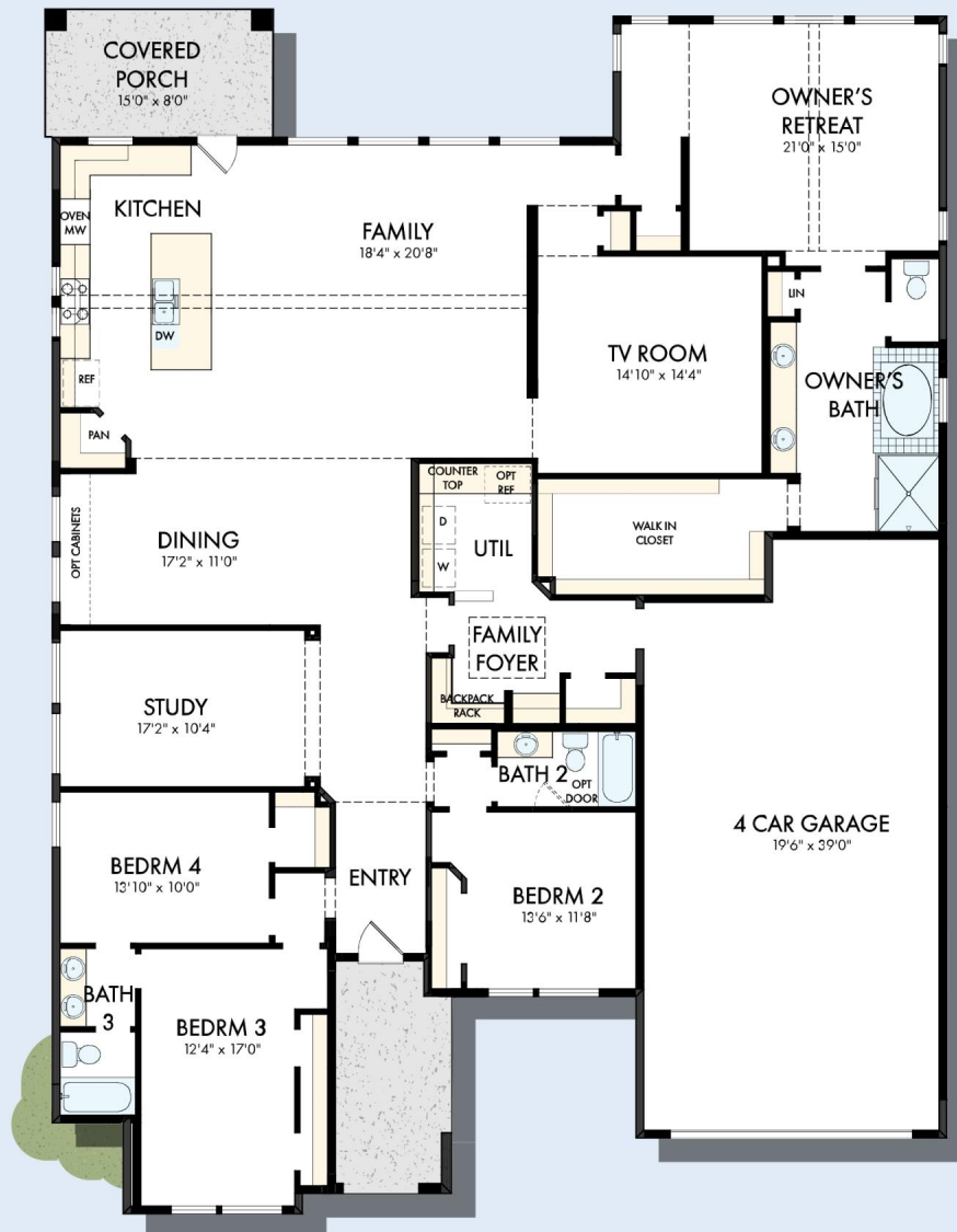
OPTIONAL EXTENDED COVERED PORCH AT KITCHEN
