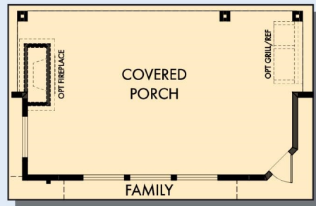
OPTIONAL EXTENDED COVERED PORCH AT FAMILY
