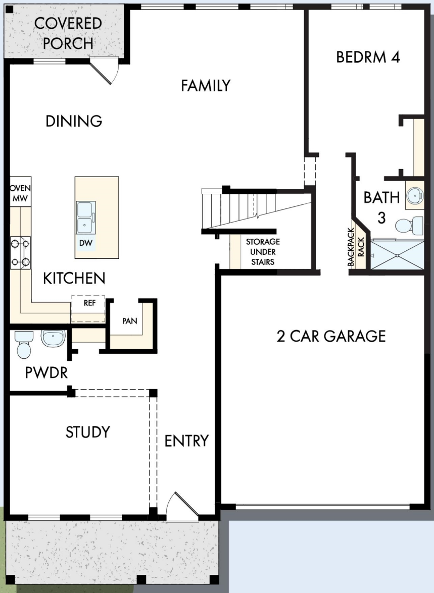
FIRST FLOOR
