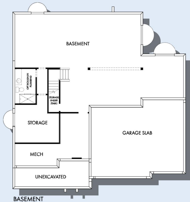
BASEMENT
