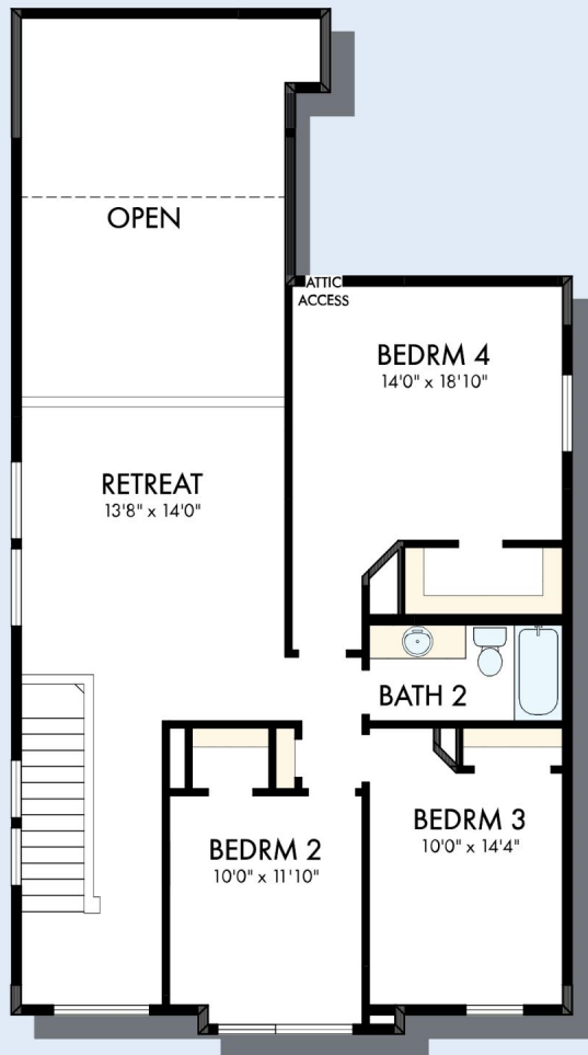
SECOND FLOOR
