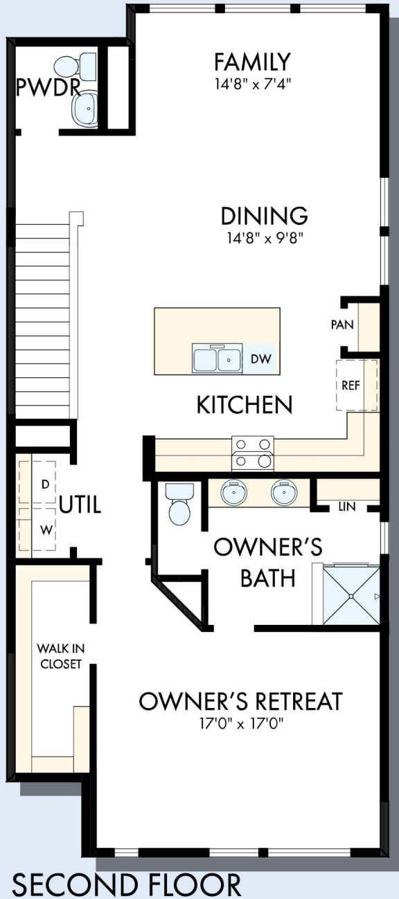
SECOND FLOOR WITH OPTIONAL THIRD FLOOR BONUS
