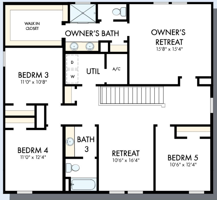
SECOND FLOOR
