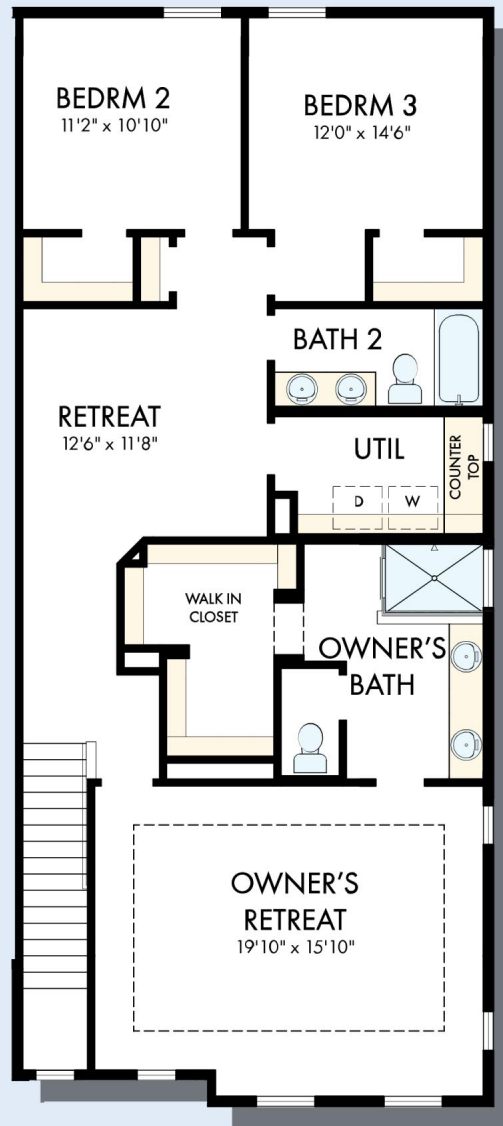
SECOND FLOOR
