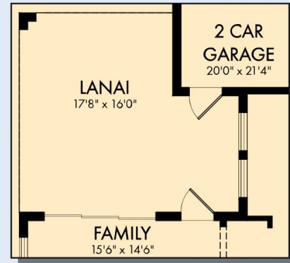
OPTIONAL EXTENDED LANAI WITH SLIDING GLASS DOOR AT FAMILY
