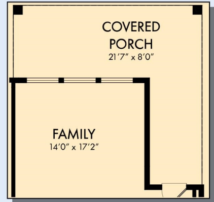
OPTIONAL EXTENDED COVERED PORCH
