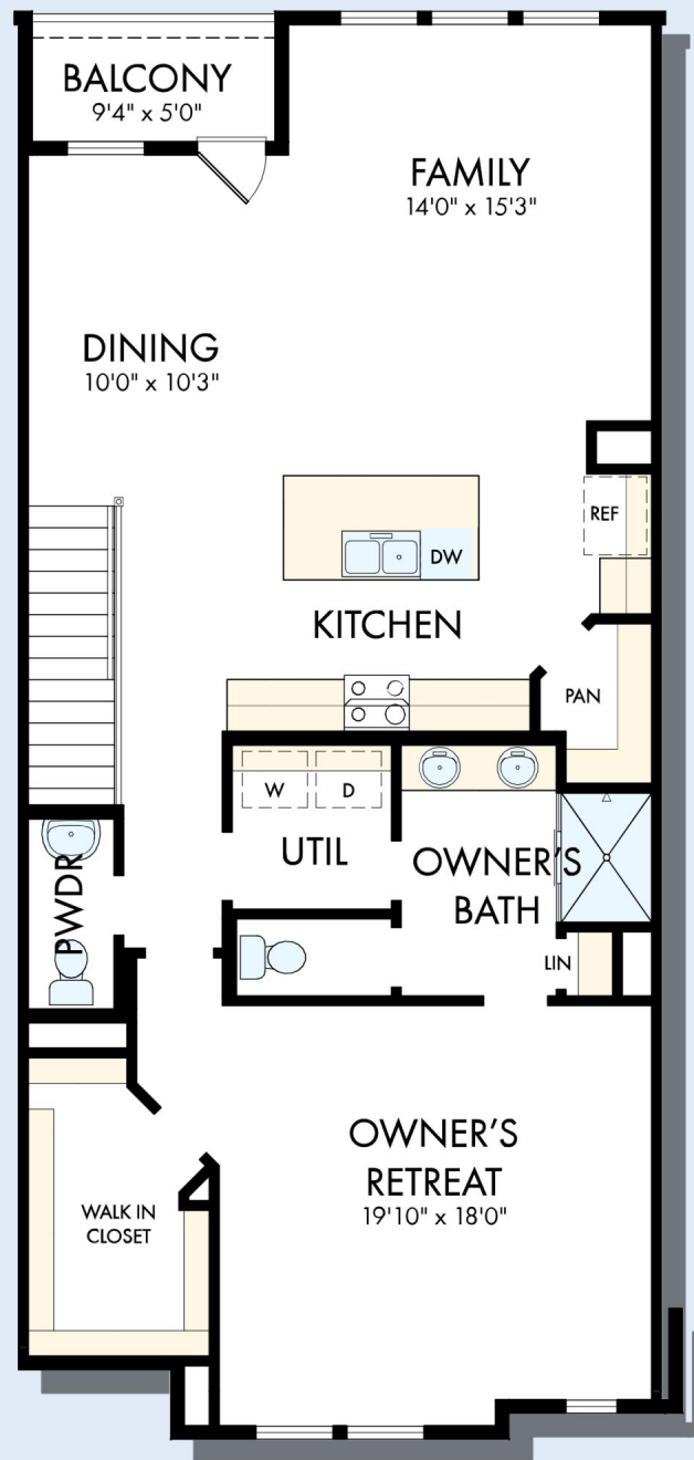
SECOND FLOOR
