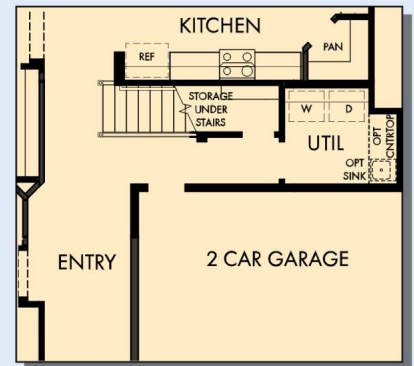
FIRST FLOOR WITH OPTIONAL SECOND FLOOR BONUS
