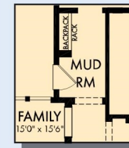
OPTIONAL MUDROOM AT REAR PORCH
