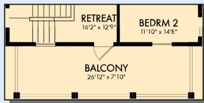
OPTIONAL BALCONY AT RETREAT
