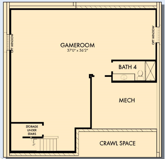
OPTIONAL GAMEROOM WITH BATH 4 AT BASEMENT
