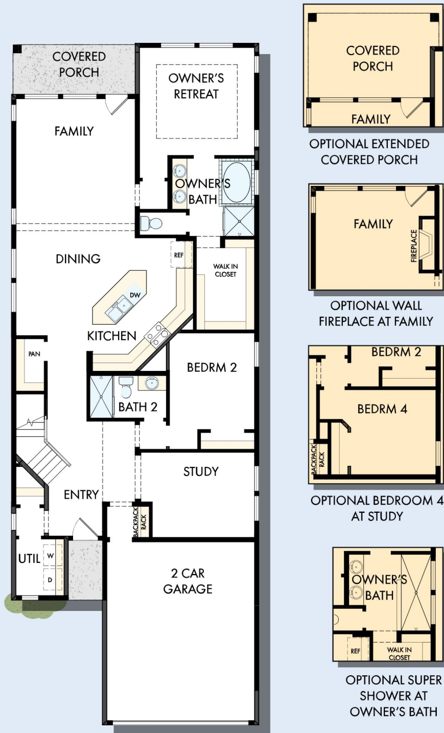
FIRST FLOOR
