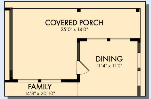
OPTIONAL EXTENDED COVERED PORCH
